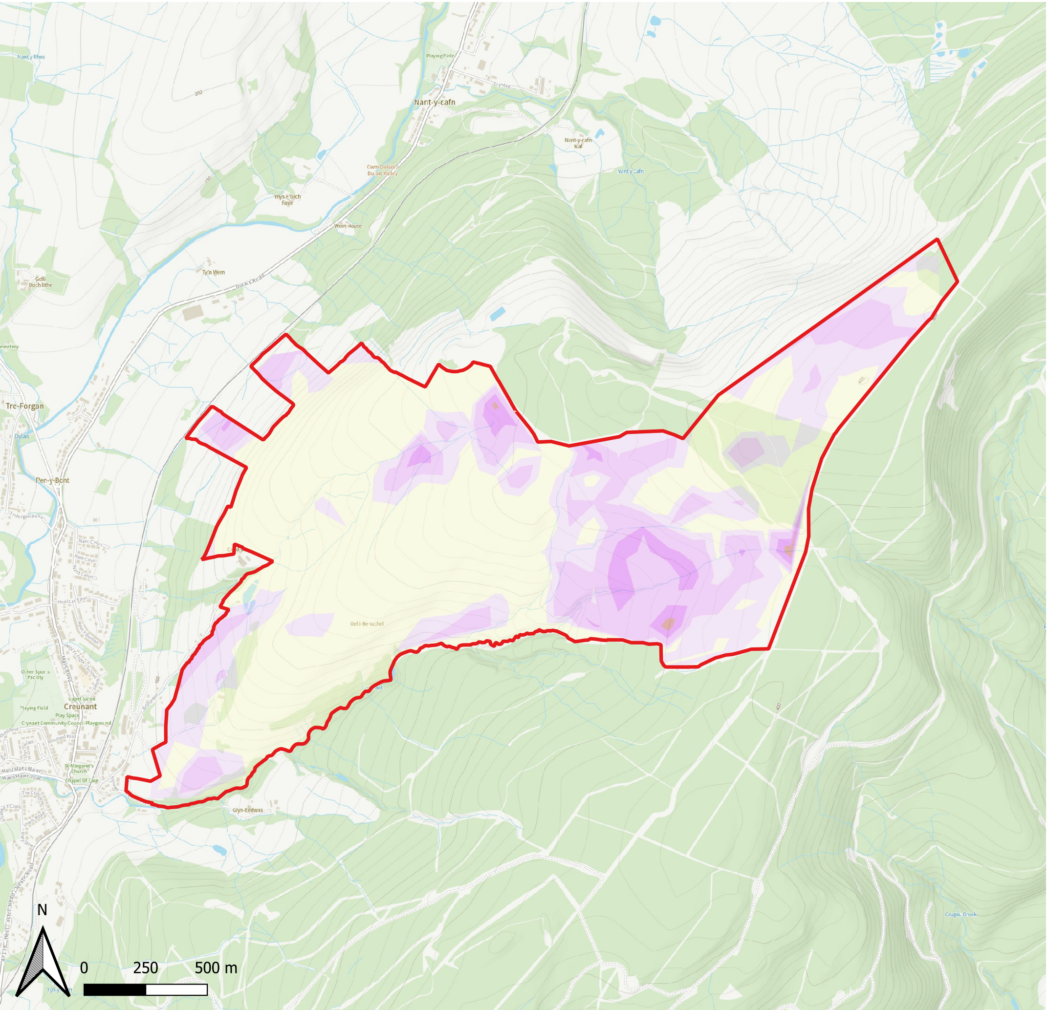
Figure 7.3: Peat Depths
