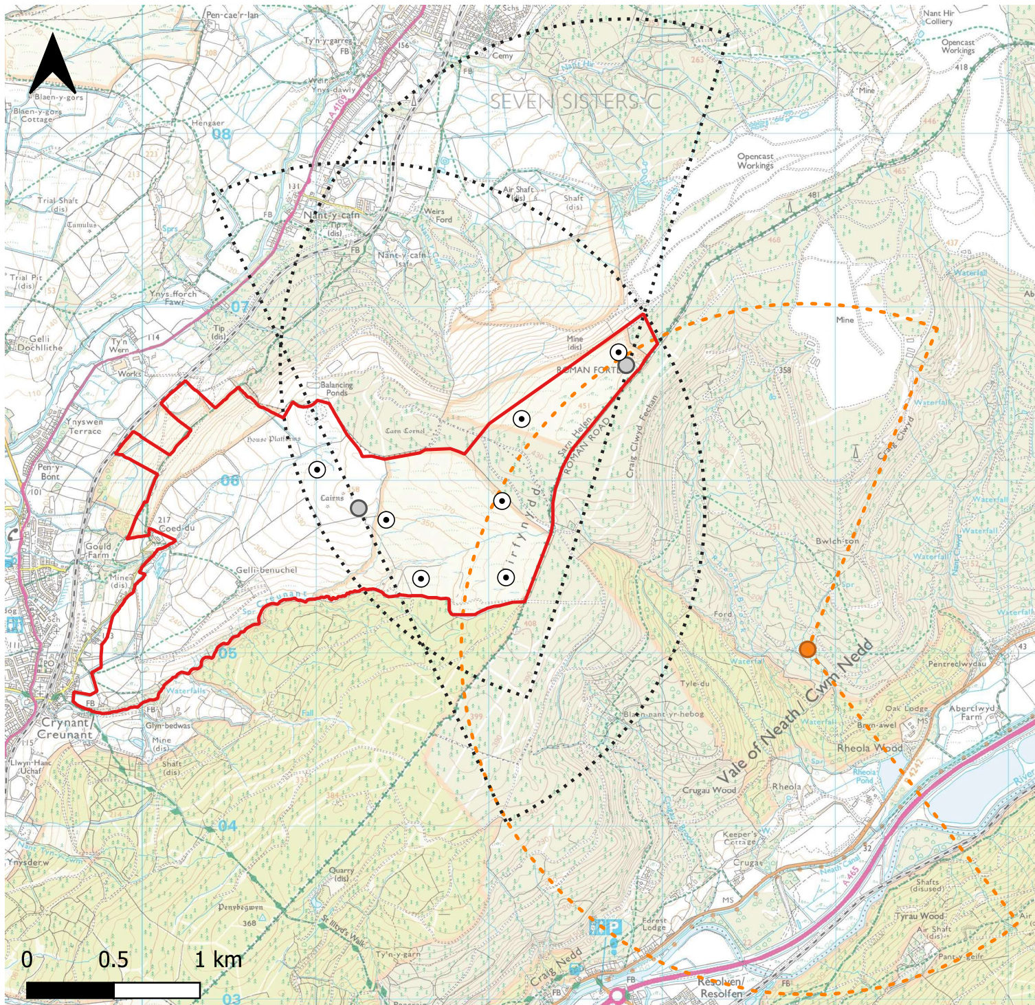
Figure 9.1: VP Locations
