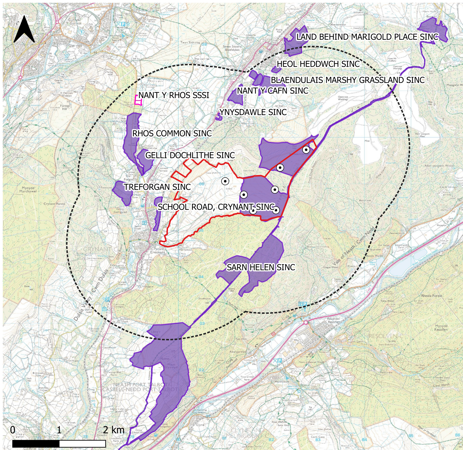
Figure 8.1: Designated Sites
