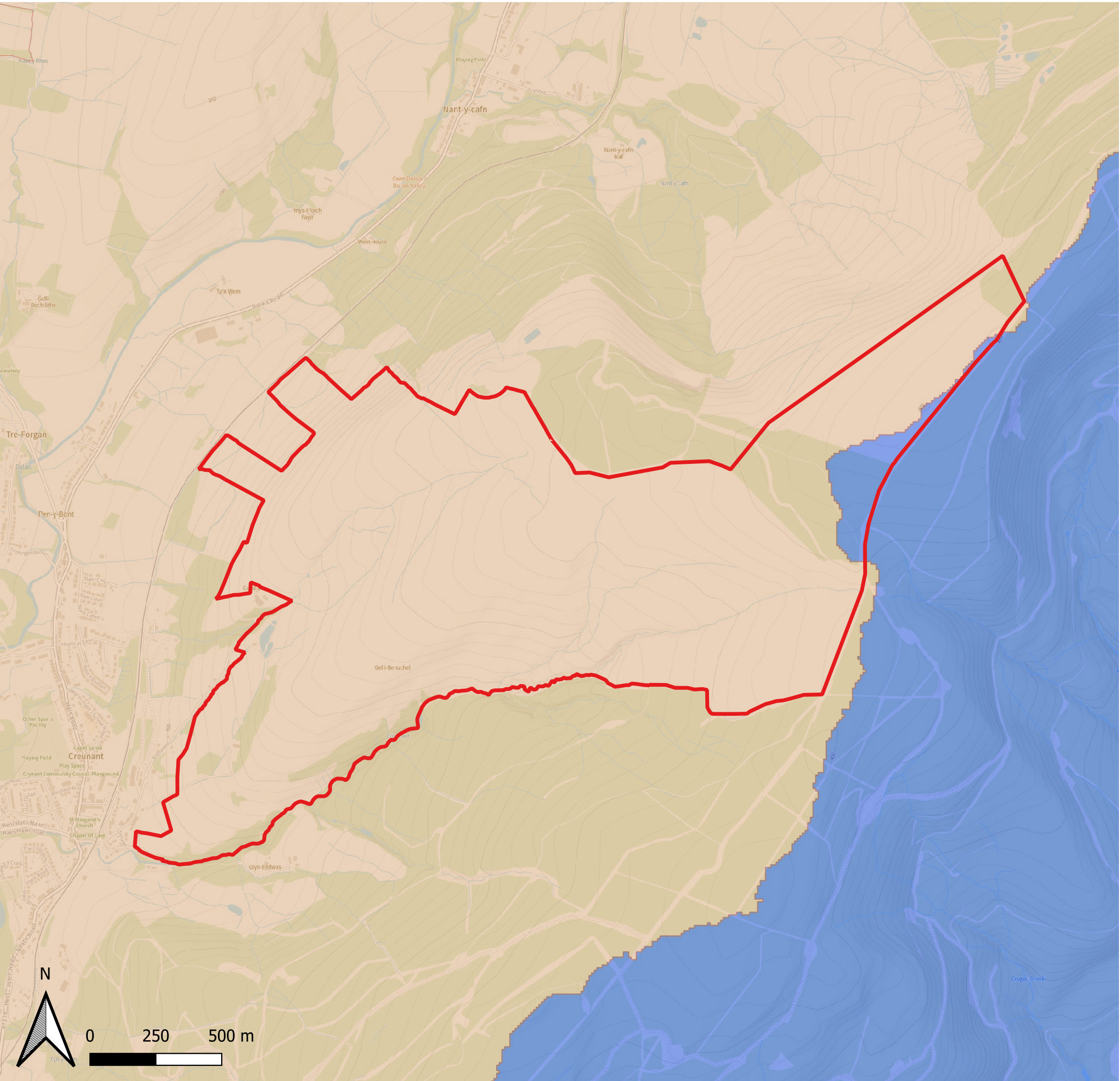
Figure 7.1: River Catchments
