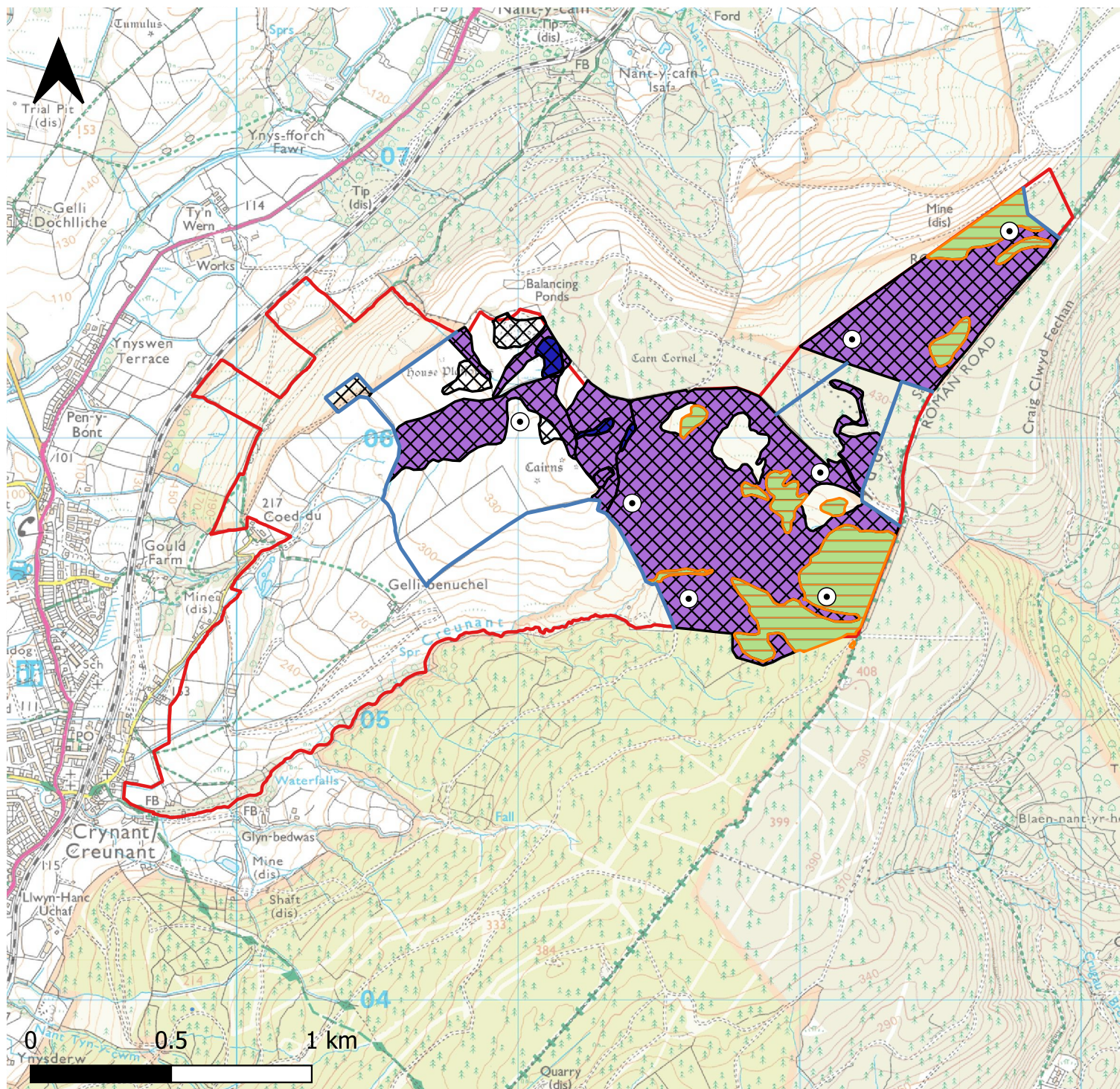
Figure 8.2: Habitats
