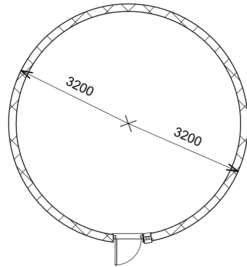
1 ground floor 1 : 100
